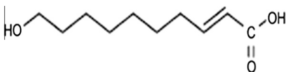
Fig. 4 – trans -10-hydroxy-2-decenoic acid (10-HDA).
